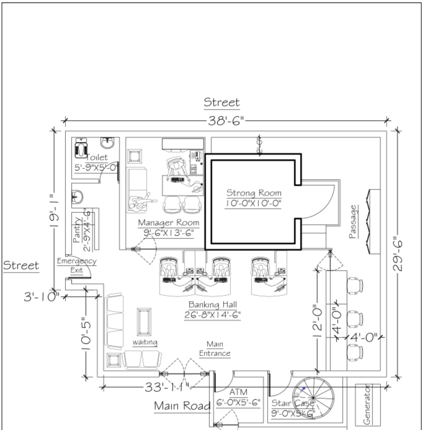
Proposed Layout Plan (Ground Floor) Branch Code # 0151 Name: Muslim Bagh Branch Quetta Region
