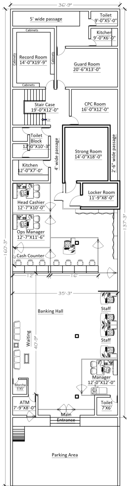
GROUND FLOOR (PROPOSED) Total Area = 5,890 SFT
