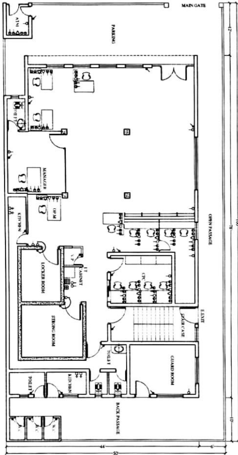
GROUND FLOOR ELECTRICAL PLAN FOR POWER SOCKETS, TELEPHONE & LAN NODES
