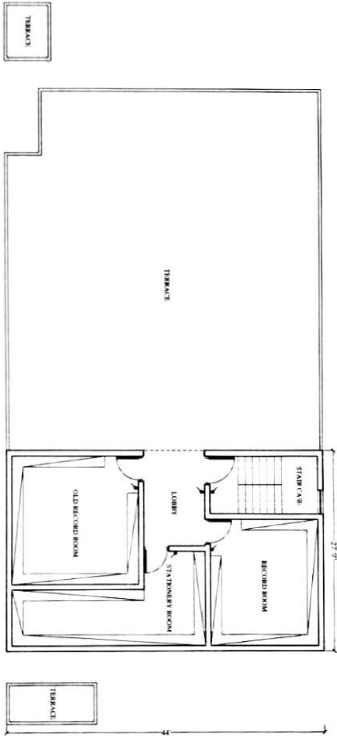
FIRST FLOOR ELECTRICAL PLAN FOR POWER SOCKETS, TELEPHONE & LAN NODES
