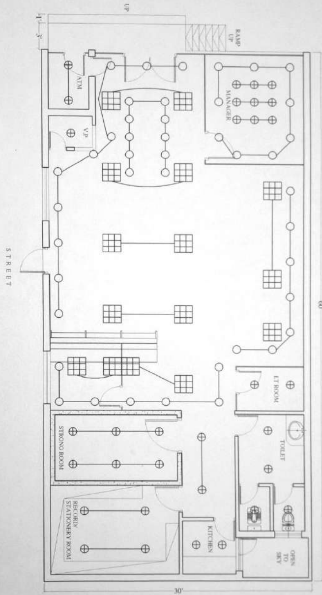
GROUND FLOOR ELECTRICAL POINTS WIRING PLAN COVERED AREA = 1800 SFT.
